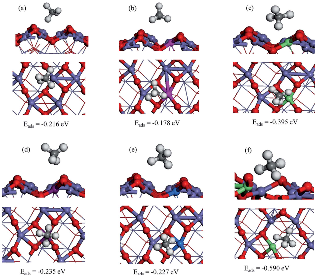
Fig. 2 Optimized structure of CH 4 adsorption on M/α-Fe 2 O 3 (110) surfaces: (a) α-Fe 2 O 3 (110), (b) Ag/α-Fe 2 O 3 (110), (c) Ir/α-Fe 2 O 3 (110), (d) Co/α-Fe 2 O 3 (110), (e) Cu/α-Fe 2 O 3 (110), and (f) Ir/α-Fe 2 O 3 (110)–O v surfaces.
