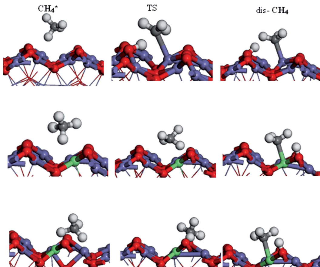
Fig. 6 Side view of initial, transition, and intermediate states of \text{CH}_4 oxidation on \alpha\text{-Fe}_2\text{O}_3(110) , \text{Ir}/\alpha\text{-Fe}_2\text{O}_3(110) , and \text{Ir}/\alpha\text{-Fe}_2\text{O}_3(110)\text{-O}_\text{V} surfaces.
