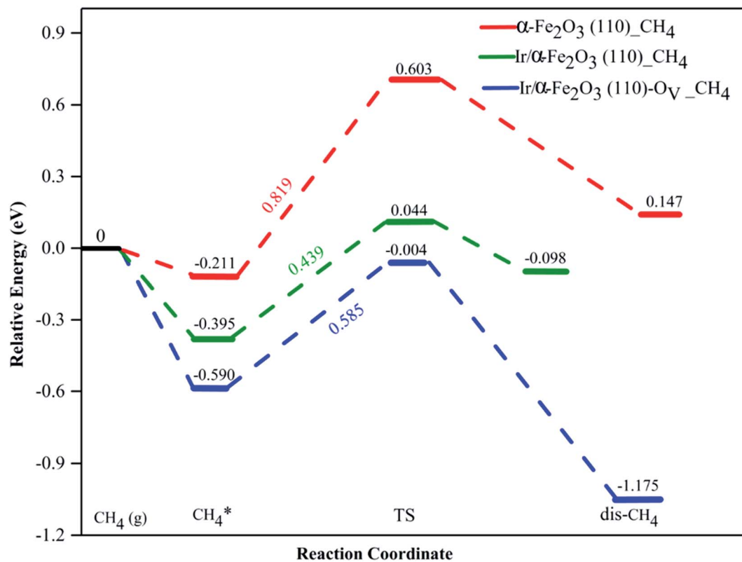
Fig. 5 Potential energy profile of \text{CH}_4 activation on \alpha\text{-Fe}_2\text{O}_3(110) (red dash line), \text{Ir}/\alpha\text{-Fe}_2\text{O}_3(110) (green dash line), and \text{Ir}/\alpha\text{-Fe}_2\text{O}_3(110)\text{-O}_\text{V} surfaces (blue dash line).
