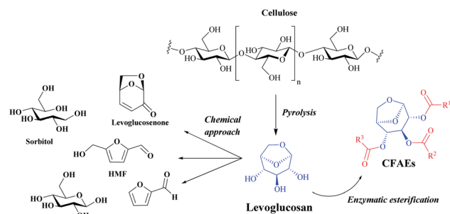
Fig. 1 General representation for highly valued products obtained by chemical and biochemical transformation of LG.
