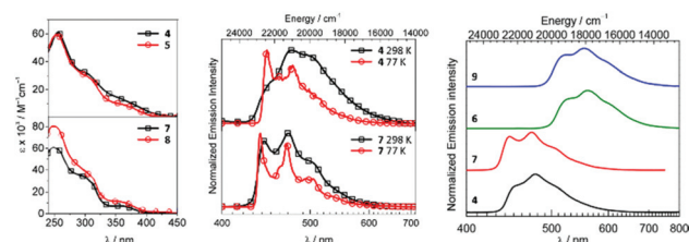
Fig. 5 (Left): UV-vis spectra of 4 , 5 , 7 , and 8 in CH 2 Cl 2 ; (centre): normalised emission spectra of 4 and 7 in CH 2 Cl 2 at RT and in CH 2 Cl 2 /toluene at 77 K; (right): normalised emission spectra of 4 , 6 , 7 , and 9 in the PMMA film (2 wt%) at RT. Adapted with permission from ref. 56 and 77. Copyright (2017, 2018) American Chemical Society.
