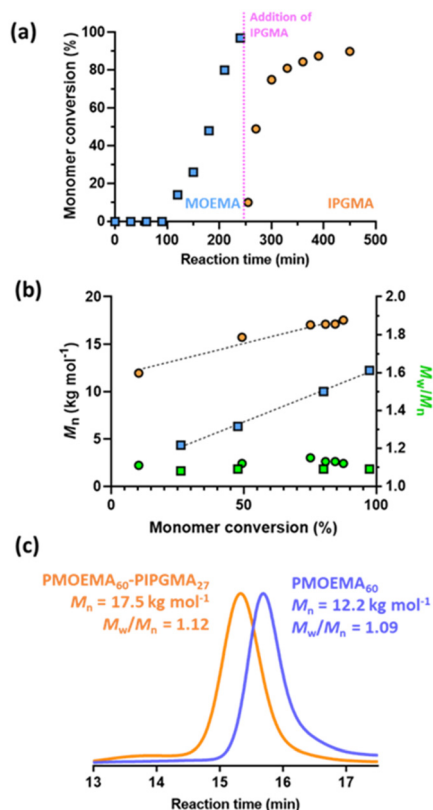
Fig. 7 Kinetic data obtained for the RAFT aqueous emulsion polymerization of MOEMA using a cationic MPETTC RAFT agent at 56 °C and the subsequent extension of the PEOEMA chains with IPGMA: (a) monomer conversion vs. time curves; (b) evolution in number-average molecular weight ( M_n ) and dispersity ( M_w/M_n ) with monomer conversion. Polymerization conditions: [MOEMA]/[MPETTC] molar ratio = 60, [IPGMA]/[PEOEMA 60 ] = 27, [MPETTC]/[AIBA] molar ratio = 5.0, targeting 7.5% w/w solids at pH 3. (c) DMF GPC curves recorded for PEOEMA 60 and PEOEMA 60 -PIPGMA 27 . Molecular weight data are expressed relative to a series of near-monodisperse poly(methyl methacrylate) calibration standards.
