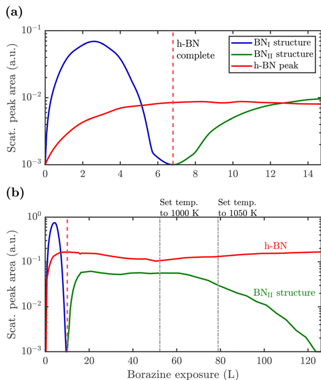
Fig. 5 Peak areas of the characteristic diffraction peaks representing the different structures versus borazine exposure. After the \text{BN}_\text{I} structure has disappeared the h-BN peak saturates giving rise to a conversion and further exposure leads to the rise of the \text{BN}_\text{II} structure. Due to a higher substrate temperature of 915 K in (a), the \text{BN}_\text{I} structure disappears already after an exposure of \approx 7 L compared to 10 L at 880 K in (b), thus indicating a kinetically driven conversion. Dosing in (b) is then further continued with subsequent changes of the surface temperature as stated above the diagram. After long enough exposure the \text{BN}_\text{II} structure disappears leaving a strong h-BN intensity behind.
