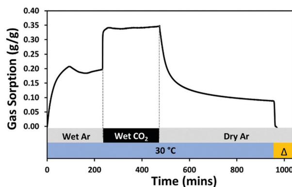
Fig. 14 TGA- \text{CO}_2 and \text{H}_2\text{O} sorption ( \text{g g}^{-1} ) of 10 : 1 (R) in humid environment at 30 °C, under 80 \text{ml min}^{-1} \text{CO}_2 , 10 \text{ml min}^{-1} Ar and 21.4% RH.
