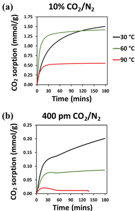
Fig. 13 TGA- \text{CO}_2 sorption ( \text{mmol g}^{-1} ) of 10 : 1 (R), in (a) 1 atm 10% \text{CO}_2/\text{N}_2 (b) 1 atm 400 ppm \text{CO}_2/\text{N}_2 .
