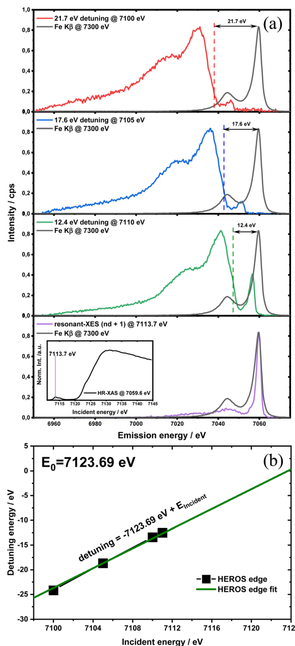
Fig. 3 (a) Detuning parameter \delta E in the function of incident energy and position changes of HEROS spectra with respect to nXES for \text{FeCl}_3 . The inset shows an incident energy of 7113.7 eV on the HR-XAS spectrum (@7059.6 eV) for which a resonant-XES spectrum was collected; (b) \delta E(E_{\text{inc}}) relation with extrapolation to \delta E = 0 .
