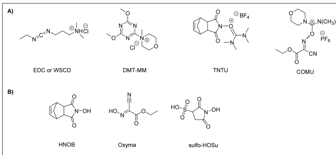
Fig. 2 (A) Efficient coupling reagents for aqueous solid-phase peptide synthesis. (B) Common additives used in coupling reactions of aqueous solid-phase peptide synthesis. EDC = N -ethyl- N' -(3-dimethylaminopropyl)carbodiimide hydrochloride; WSCD = water-soluble carbodiimide; COMU = (1-cyano-2-ethoxy-2-oxoethylideneaminoxy)dimethylamino-morpholino-carbenium hexafluorophosphate.
