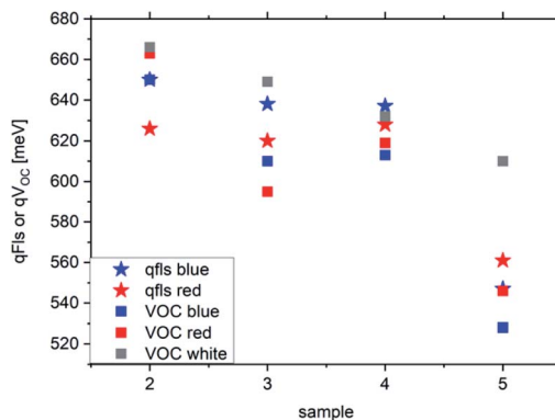
Fig. 7 qFIs and V_{OC} for the \text{Cu}(\text{In,Ga})(\text{S,Se})_2 samples illuminated with a red laser (660 nm), a blue laser (405 nm) or a simulated AM1.5 spectrum (white).
