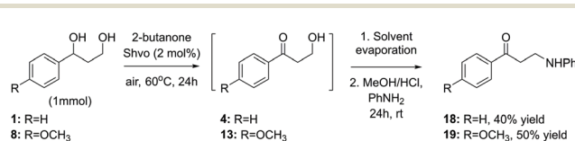
Scheme 7 Two-step diol amination procedure involving solvent replacement.
