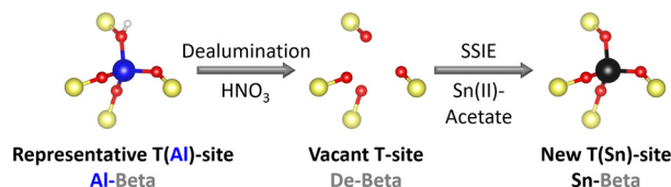
Fig. 2 Scheme of the two step preparation procedure of Sn-Beta zeolites. SSIE = solid state ion exchange.
