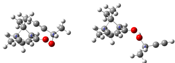
Fig. 1 The structural characterization of the lowest energy isomers of the 1 : 1 complexes formed between verbenone and butynol is illustrated. The two hydrogen bond positions are shown in the top panel (A). Most quantum chemistry methods identify two equilibrium geometries for the dihedral angle around the O...O axis of the hydrogen bond as shown in panel (B). The structures shown in this figure are equilibrium geometries from the B3LYP GD3BJ def2TZVP calculation set.
