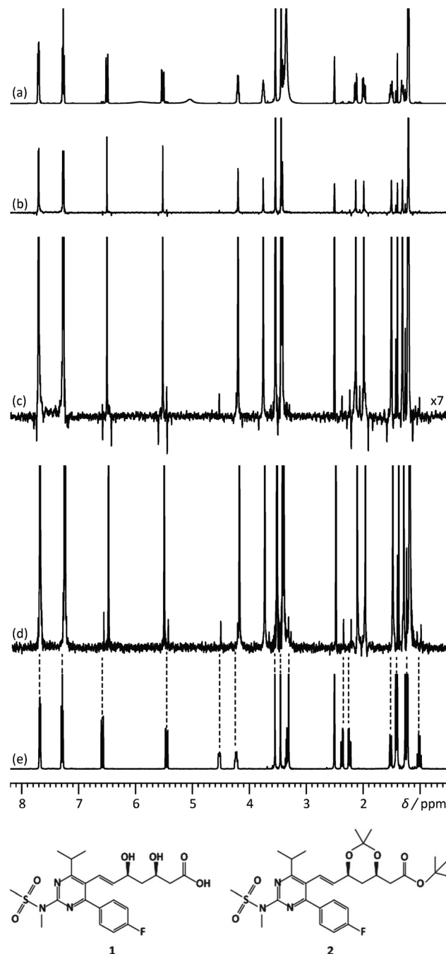
Fig. 2 500 MHz (a) 1D 1 H spectrum, (b) 1 H pure shift spectrum recorded using the unmodified Zangger–Sterk pulse sequence, (c) vertical expansion of the spectrum (b) and (d) 1 H pure shift spectrum acquired with the pulse sequence modified to remove sidebands, for a mixture containing rosvastatin (1) and 2.8% of its precursor BEM (2). (e) 1D 1 H spectrum of BEM. Spectra c and d were acquired in approximately 9 h with an sw1 of 39.0625 Hz and 16 chunks using an RSNOB spatially selective spin inversion element with a peak RF amplitude of 47 Hz. Reproduced from ref. 25 with permission from the Royal Society of Chemistry.
