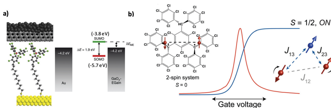
Fig. 3 (a) Scheme of the Au/S-alkyl-PTM SAM/GaO x /EGaIn and the corresponding energy level diagram. Reprinted with permission from ref. 49. Copyright 2016 Nature Group. (b) Left: Structure and magnetism schematics of the neutral diradical investigated. The red dots and the dashed lines are the radical spins (2-spin system as synthesised, S = 0 ) and the exchange interactions, respectively. Right: Differential conductance (red) and corresponding redox center spin values (blue) as a function of gate voltage. The added electron is marked as the blue dot (3-spin system, S = 1/2 ). Reprinted with permission from ref. 52. Copyright 2017 ACS Publications.
