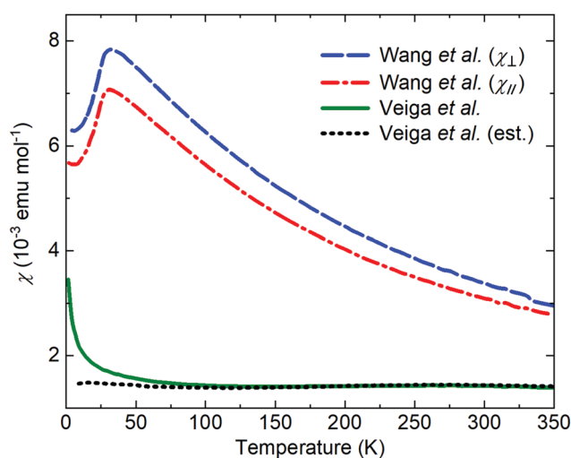
Fig. 7 The reported magnetic properties of \text{Na}_2\text{RuO}_3 provide an example of conflicting measurements of a quantum material. In 2014, Wang et al. 136 reported the susceptibility of a single-crystal sample oriented with the plane of the \text{RuO}_6 layers perpendicular to (blue) or parallel to (red) a 3 T applied field. In 2020, Veiga et al. 132 reported the susceptibility of a polycrystalline sample in a 1 T applied field (green; the dotted line shows an estimated intrinsic susceptibility obtained by subtracting a Curie-like impurity contribution). Recent studies of polycrystalline samples have shown that \text{Na}_2\text{RuO}_3 is not stable in air at ambient conditions and that carefully handled samples do not display long-range magnetic order. 132,137
