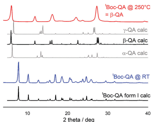
Fig. 2 Comparison of the experimental powder XRD patterns with those calculated on the basis of the single-crystal data for compounds. 34 Top: thermal deprotection of a polycrystalline sample of 'Boc-QA leads to formation of \beta -QA.
