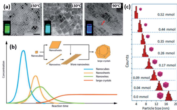
Fig. 7 (a) TEM images of \text{CsPbBr}_3 NCs grown at different temperatures with photos of the solutions under UV-illumination in the inset of the figures. The scale bar is 50 nm. (b) A sketch illustrating the morphology evolution during the synthesis of \text{CsPbBr}_3 NCs by HI approach. (c) Size distribution histogram of \text{CsPbBr}_3 nanocubes obtained at 160 °C from the reaction with varying amounts of oleylammonium bromide. Panels (a), (b) and (c) are adapted with permission from ref. 136, 138 and 140, respectively.
