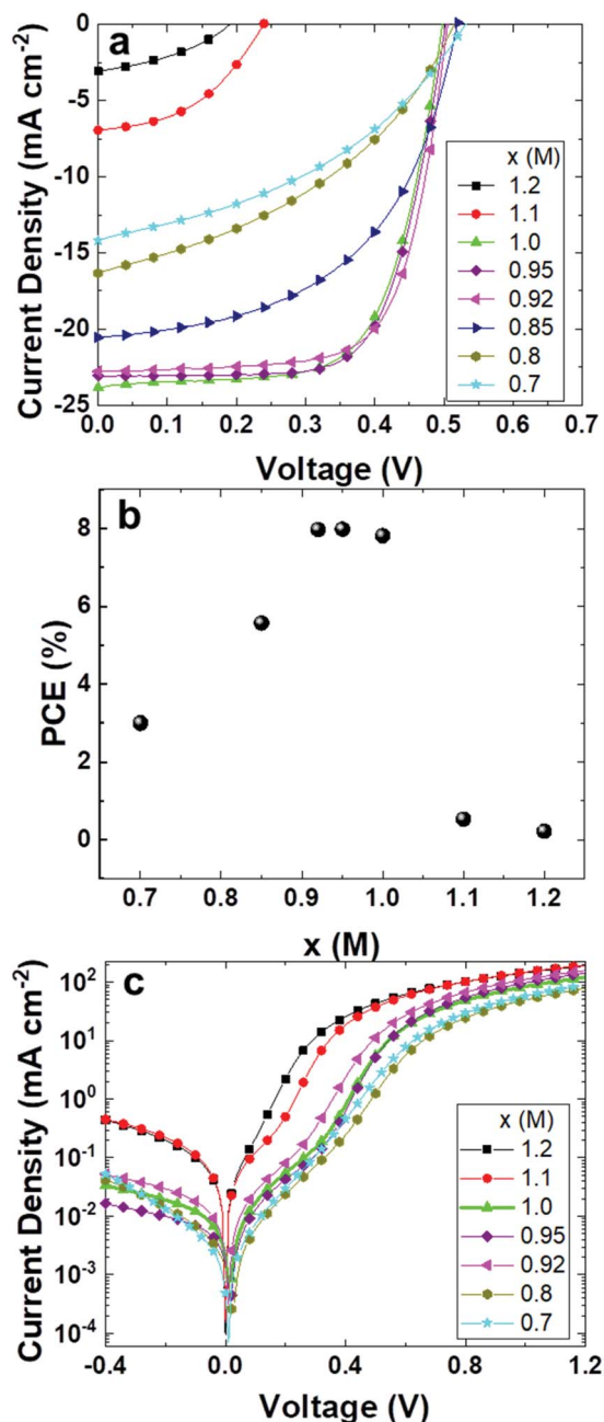
Fig. 6 \text{PEA}_{0.08}\text{FA}_x\text{SnI}_3 based devices. (a) J - V curves under AM 1.5G conditions, (b) PCE versus FA concentration and (c) J - V curves of the solar cells under dark conditions. Displayed results are coming from a batch of consistent samples.
