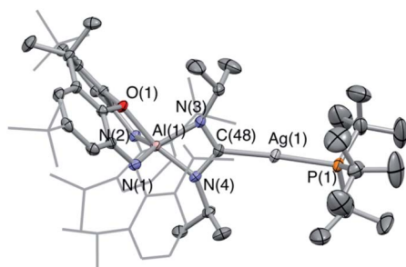
Fig. 4 Molecular structure of 5-Ag in the solid state as determined by X-ray crystallography. Thermal ellipsoids set at the 50% probability level. Hydrogen atoms omitted and {}^1\text{Pr}/{}^4\text{tBu} shown in wireframe for clarity. Key bond lengths (Å) and angles (°): Ag(1)–C(48): 2.118(2), Ag(1)–P(1): 2.3851(6), N(3)–C(48): 1.346(3), N(4)–C(48): 1.345(3).
