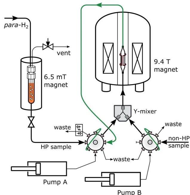
Fig. 2 Instrument for SABRE NMR measurements of ligand binding. The putative ligand interacts with para -hydrogen and polarization transfer catalyst at 6.5 mT. It is subsequently delivered to a sample loop. The ligand and protein samples are pushed by high-pressure syringe pumps through the Y-mixer, to a flow-cell in the NMR magnet, where the measurement takes place.
