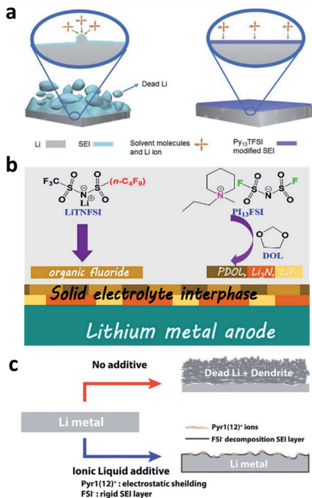
Fig. 10 The use of an ionic liquid in the electrolyte for forming nitrided interfaces on Li metal electrodes. (a) Schematic illustration of the use of the \text{Py}_{13}\text{TFSI} ionic liquid in an ether electrolyte for stabilizing the Li metal electrode; 100 reproduced with permission. Copyright 2017, John Wiley and Sons. (b) Illustration of the co-use of the \text{PL}_{13}\text{FSI} ionic liquid and \text{LiTFSI} to construct a nitrided composite SEI on the Li metal electrode; 101 reproduced with permission. Copyright 2018, American Chemical Society. (c) Illustration of the application of \text{Pyr1(12)FSI} to regulate the uniform deposition of \text{Li}^+ and reduce dead Li. 102 Reproduced with permission. Copyright 2018, John Wiley and Sons.
