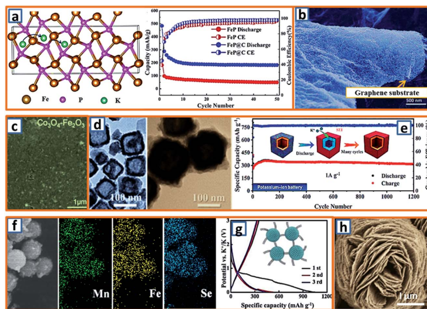
Fig. 12 Potassium storage chemistry and applications of conversion-type anodes. (a) Diffusion pathway of the K + ions in the FeP structure, and its corresponding potassium storage performance. Reproduced with permission. 18 Copyright 2019, American Chemical Society. (b) SEM image of CoS@G. Reproduced with permission. 37 Copyright 2017, Wiley. (c) Surface morphology of the conversion-type Co 3 O 4 -Fe 2 O 3 electrodes. Reproduced with permission. 14 Copyright 2017, The Royal Society of Chemistry. (d) TEM of the synthesized Cu 2 S and Cu 2 S@NC, and (e) the long cycling performance of Cu 2 S@NC. Reproduced with permission. 75 Copyright 2020, American Chemical Society. (f) SEM mapping characterization and (g) discharge and charge performances of the Mn-Fe-Se/CNT composite. Reproduced with permission. 91 Copyright 2019, Elsevier. (h) SEM of the flower-like VPO 4 anode material. Reproduced with permission. 103 Copyright 2019, The Royal Society of Chemistry.
