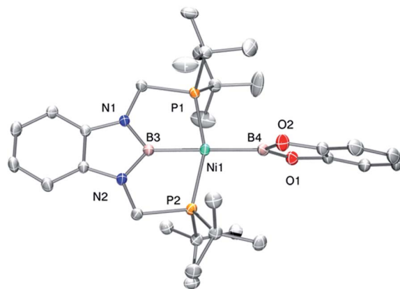
Fig. 1 Molecular structure of 3 (H atoms omitted for clarity). Thermal ellipsoids are represented at the 50% probability level. Selected bond distances (Å) and angles (°): Ni(1)–B(4) = 2.015(2); Ni(1)–B(3) = 1.942(2); P(1)–Ni(1)–P(2) = 157.74(3); B(3)–Ni(1)–B(4) = 175.0(1).
