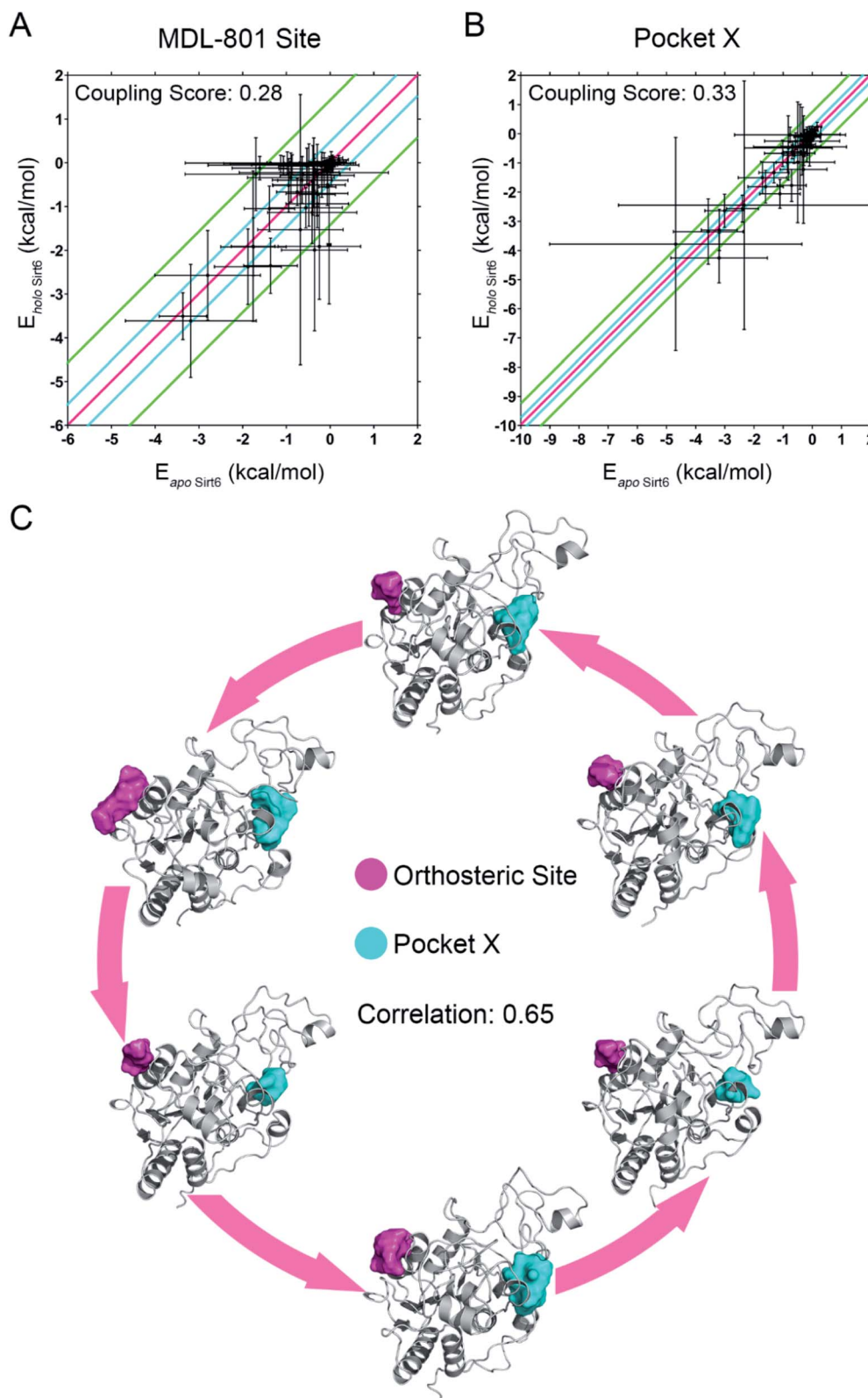
Fig. 5 Energy coupling analysis for the MDL-801 site (A) and Pocket X (B) in apo- and holo-Sirt6. Each dot represents one residue pair and its crosses indicate the corresponding standard deviations. The pink line reflects the average interaction energy changes between apo- and holo-protein. Regions between pink and cyan lines indicate small energy difference (one standard deviation, group I), regions between cyan and green lines indicate medium energy difference (three standard deviations, group II), and regions outside green lines indicate large energy difference (higher than three standard deviations, group III). (C) Correlation analysis using D3Pocket for orthosteric NAD + site (magenta) and allosteric Pocket X (cyan).
