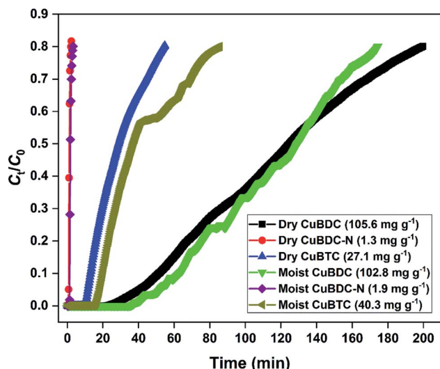
Fig. 6 H 2 S breakthrough curve of dry and moist Cu-MOFs.
