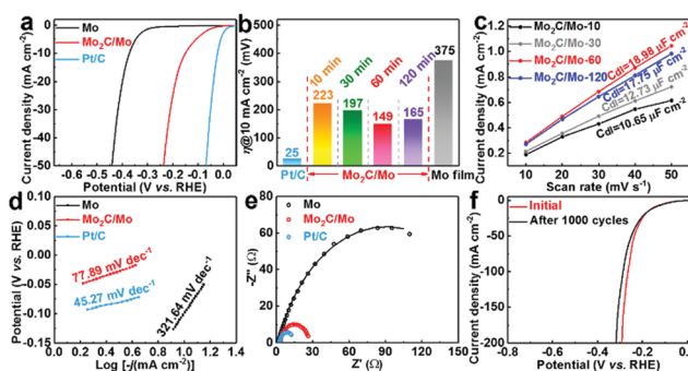
Fig. 5 (a) Polarization curves of the prepared \text{Mo}_2\text{C}/\text{Mo} -60, bare Mo plate and Pt/C catalysts at 5 \text{ mV s}^{-1} in 0.5 M \text{H}_2\text{SO}_4 at 25 °C. (b) Overpotentials at 10 \text{ mA cm}^{-2} . (c) Linear relationship between the capacitance current density and scan rate. (d) Corresponding Tafel plots and (e) EIS Nyquist plots of different samples. (f) Polarization curves of \text{Mo}_2\text{C}/\text{Mo} -60 before and after 1000 cycles.
