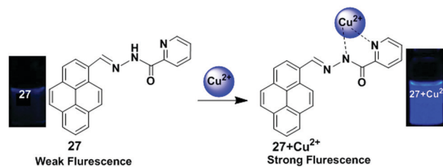
Fig. 23 Schematic representation of the sensing mechanism of probe 27 with \text{Cu}^{2+} . Reproduced from ref. 90 with permission from the Springer Nature, copyright 2012.
