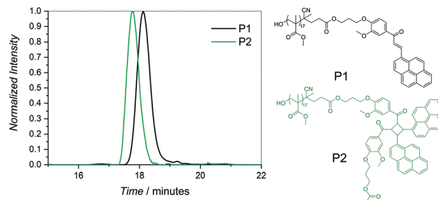
Fig. 6 XIC traces of the polymer with 17 MMA repeat units in the starting material and product shows that the product elutes before the starting material. The earlier elution time indicates that the product is larger than the starting material, which signifies the successful end group ligation of the terminal chalcone after irradiation with a green LED ( \lambda_{\text{max}} = 505 \text{ nm} ) for 3 days.
