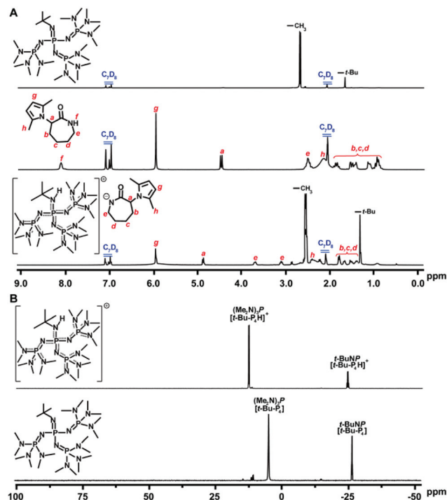
Fig. 4 (A) ^1\text{H} NMR spectra (toluene- d_8 , 25 °C) of the reaction between t\text{-BuP}_4 and M5 (1:1). (B) ^{31}\text{P} NMR spectra (toluene- d_8 , 25 °C) of the reaction between t\text{-BuP}_4 and M5 (1:1). Reproduced from ref. 26 with permission from the American Chemical Society, copyright 2017.
