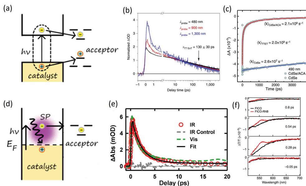
Fig. 3 (a) Energy transfer mechanism, HOMO and LOMO or the triplet states of the molecular acceptor needs to lie within the bandgap of photocatalyst; (b) energy transfer dynamics in [2 + 2] cycloaddition reaction catalyzed by CdS quantum dots. The figure was adapted from ref. 20 with permission from Springer Nature (c) triplet energy transfer dynamics in CdSe/ACA system. The figure was adapted from ref. 63 with permission from AAAS (d) hot carrier transfer mechanism, hot carriers can be generated by plasmon resonance and thus transfer to substrate; (e) dynamics of plasmon induced hot electron transfer in Au–CdS. Plasmon-induced hot electron transfer time of 20 fs is observed with 1.45 ps recombination time. The figure was adapted from ref. 66 with permission from AAAS. (f) Dynamics of hot carrier transfer from CdO quantum dots to surface anchored rhodamine B molecules. Ultrafast hot carrier transfer of <50 fs is observed. The figure was adapted from ref. 67 with permission from Springer Nature.
