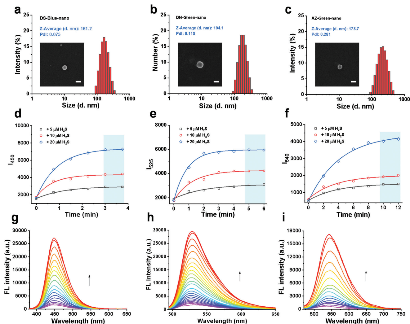
Fig. 3 Construction and validation of PTC-based nanoprobe of DS-Blue-Nano, DN-Green-Nano, and AZ-Green-Nano. (a–c) Particle size distributions of DS-Blue-Nano, DN-Green-Nano, and AZ-Green-Nano measured by DLS, PDI < 0.3. The insets in Fig. 3a–c show the SEM images of the samples and scale bars correspond to 200 nm; (d–f) time-course of DS-Blue-Nano, DN-Green-Nano, and AZ-Green-Nano (10 \mu\text{M} for each) with the addition of \text{H}_2\text{S} (5 \mu\text{M} , black; 10 \mu\text{M} , red; 20 \mu\text{M} , blue) in PBS (10 mM, pH 7.4); (g–i) fluorescent titration of DS-Blue-Nano, DN-Green-Nano, and AZ-Green-Nano (10 \mu\text{M} for each) in response to different concentrations of \text{H}_2\text{S} in PBS (10 mM, pH 7.4).
