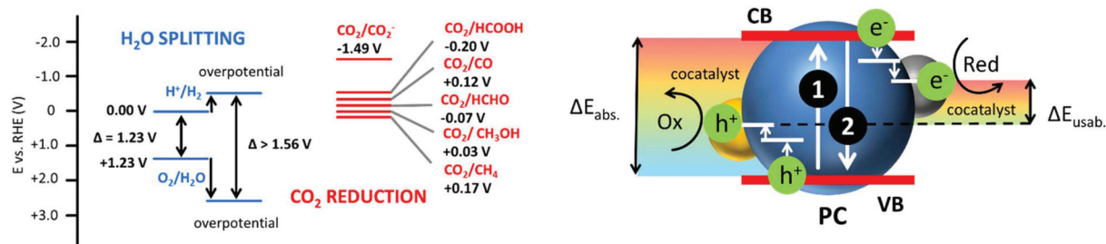
Fig. 1 Left. Simplified energy diagrams for water splitting and \text{CO}_2 photoreduction. The actual energy need \Delta G for water splitting is only 1.23 V that corresponds to just about 1000 nm and hence to NIR region photons. Nevertheless, the overpotential for this multistep process is considerable and higher energy is needed even in the case of the use of cocatalyst for reduction and oxidation. Additionally, as shown on the right, photon energy is absorbed by the PC ( \Delta E_{\text{abs.}} ) transferring an electron from the valence band (VB) to the conduction band (CB), therefore producing the electron–hole pair (process 1). Nevertheless, even in the case of poor charge recombination (process 2), several processes occur before the separated and trapped electron are available for the reaction (including charge transfer to the cocatalysts). This reduces the amount of energy actually available for redox ( \Delta E_{\text{usab.}} ).
