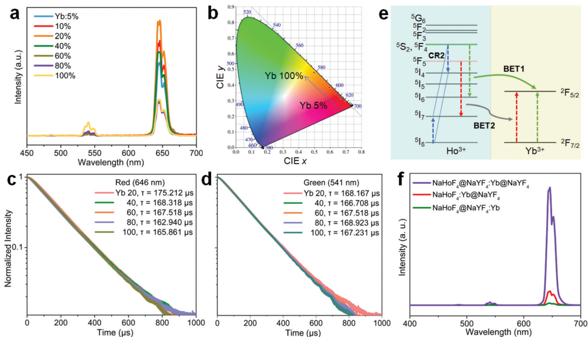
Fig. 4 (a) Upconversion emission spectra of \text{NaHoF}_4@ \text{NaF}_4\text{:Yb(5–100 mol\%)}@ \text{NaF}_4 core-shell nanoparticles under 980 nm excitation. (b) CIE coordinates of the emissions from (a) samples. (c and d) Decay curves of the upconversion emissions measured at (c) 646 nm and (d) 541 nm under pulsed 980 nm excitation. (e) Possible back energy transfer processes for decreasing the red and green upconversion emissions under 980 nm excitation. (f) Comparison of the upconversion emission spectra of the as-prepared \text{NaHoF}_4@ \text{NaF}_4\text{:Yb(20 mol\%)}@ \text{NaF}_4 core-shell, \text{NaHoF}_4\text{:Yb(20 mol\%)}@ \text{NaF}_4 core-shell, and \text{NaHoF}_4@ \text{NaF}_4\text{:Yb(20 mol\%)}@ \text{NaF}_4 core-shell-shell nanoparticles under 980 nm excitation.
