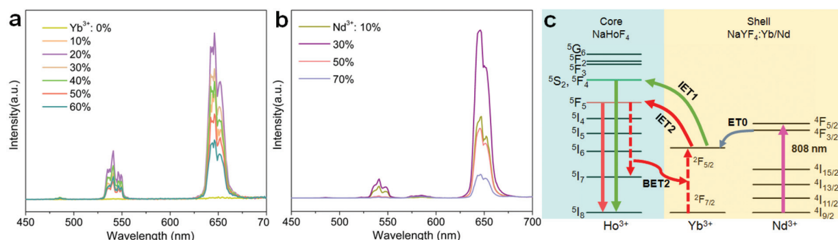
Fig. 5 (a and b) Upconversion emission spectra of \text{NaHoF}_4@\text{NaYF}_4:\text{Yb}(0-60 \text{ mol}\%) and \text{NaHoF}_4@\text{NaYF}_4:\text{Yb}(20 \text{ mol}\%)/\text{Nd}(10-70 \text{ mol}\%) core-shell nanoparticles under 980 and 808 nm excitations, respectively. (c) Schematic of the energy transport processes in the \text{Nd}^{3+} -sensitized upconversion system.
