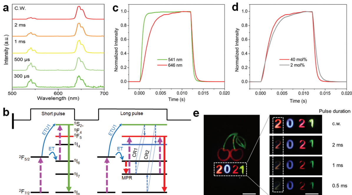
Fig. 7 (a) Upconversion emission spectra of \text{NaYF}_4:\text{Ho}(40\text{ mol}\%)@ \text{NaYF}_4:\text{Yb}(60\text{ mol}\%)@ \text{NaYF}_4 core–shell–shell nanoparticles under pulsed 980 nm excitation with a tuning of the pulse duration. (b) Schematic of the possible processes for the reduction of the red upconversion under non-steady state excitation. (c) Time-dependent emission profiles of \text{Ho}^{3+} at 541 and 646 nm of (a) sample under 980 nm irradiation with a pulse duration of 12 ms (50 Hz). (d) A comparison of the time-dependent red upconversion emission profiles from the (a) sample and \text{NaYF}_4:\text{Yb}/\text{Ho}(20/2\text{ mol}\%)@ \text{NaYF}_4 core–shell nanoparticles. (e) Schematic of decoding the concealed information on the cherry pattern under pulsed 980 nm irradiation (right panels) in which only the initial number “2” shows a color change with reducing the pulse duration. Scale bars, 0.5 cm.
