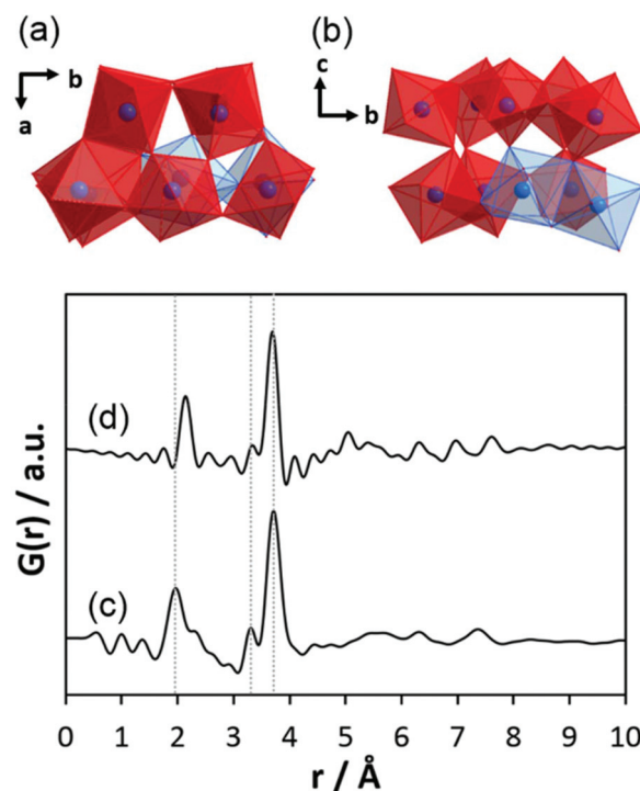
Fig. 11 Cluster model derived from cutting a part of the crystal structure of \text{L-Ta}_2\text{O}_5 followed by a simple geometric optimisation: (a) top view and (b) side view. (c) Experimental PDF of h\text{-Ta}_x\text{O}_y\text{H}_z is given in comparison to (d) the PDF calculated based on this structure.
