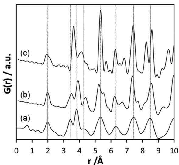
Fig. 10 (a) Experimental PDF obtained at 700 °C during heating of d\text{-Ta}_x\text{O}_y , calculated PDFs based on the structures of (b) \text{L-Ta}_2\text{O}_5 13 and (c) \beta\text{-Ta}_2\text{O}_5 . 14
