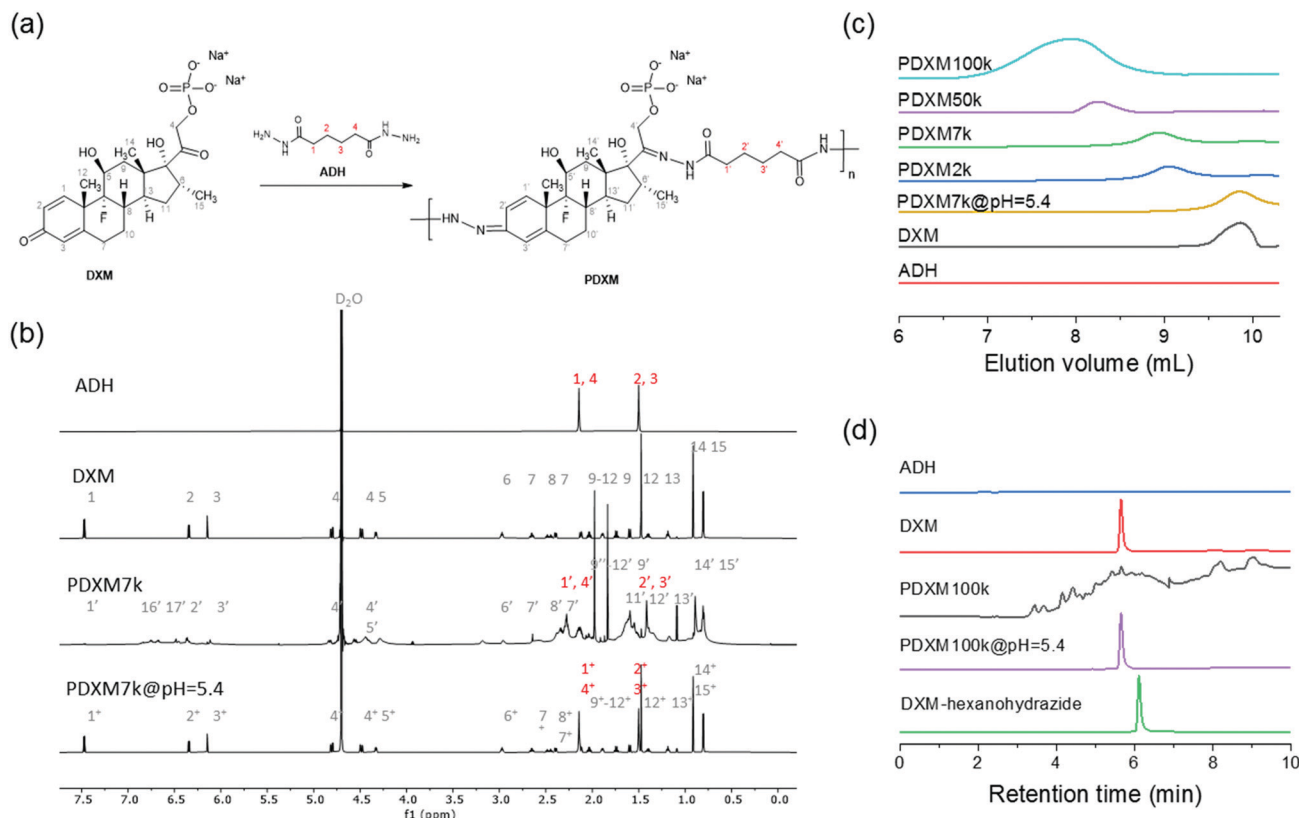
Fig. 2 (a) The route for the synthesis of PDXM prodrugs. (b) ^1\text{H} NMR (850 MHz at 298 K) spectra of ADH, DXM, PDXM7k, and PDXM7k@pH=5.4. (c) GPC chromatograms of ADH, DXM, and PDXM with different M_n , as well as degradation products of PDXM7k at pH 5.4. (d) HPLC chromatograms of ADH, DXM, PDXM100k, degradation products of PDXM100k at pH 5.4, and the DXM-hexanohydrazide conjugate.
