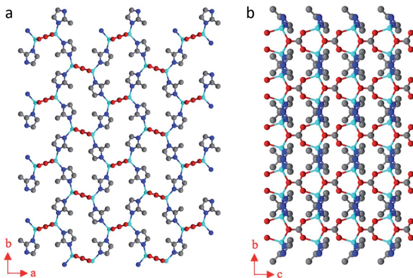
Fig. 5 The structural model of BSA@ZIF- \text{CO}_3 -1 viewed along (a) the c -axis, and (b) the a -axis. Blue spheres: N; red spheres: O; gray spheres: C; cyan spheres: Zn atoms.
