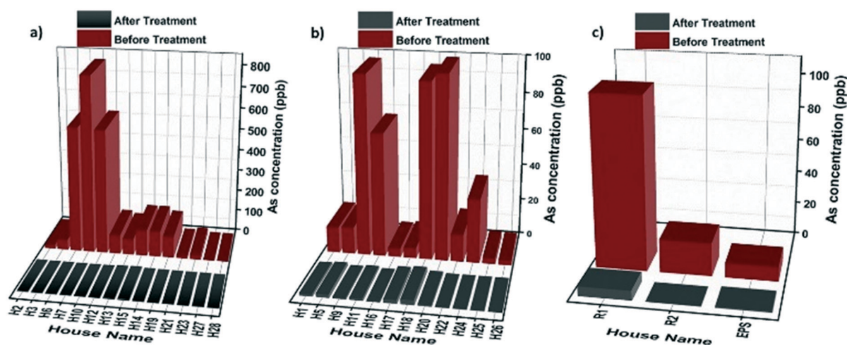
Fig. 3 (a) As concentration before and after filtration with the type I household filtration unit (Tacna: H2, H3, H10, Tacapampa: H6, H7, Inclan: H12, H13, H14, H15, Chiclayo: H21, Moquegua: H27, H28). (b) As concentration before and after filtration with the type II household filtration unit (Tacna: H1, H5, Tacapampa: H9, Inclan: H11, Chiclayo: H16, H17, H18, H20, Moquegua: H22, H24, and Cerro de Pasco: H25, H26). (c) As concentration before and after filtration with the type III community filtration unit (Tacna: EPS, Inclan: R1, Torata: R2).
