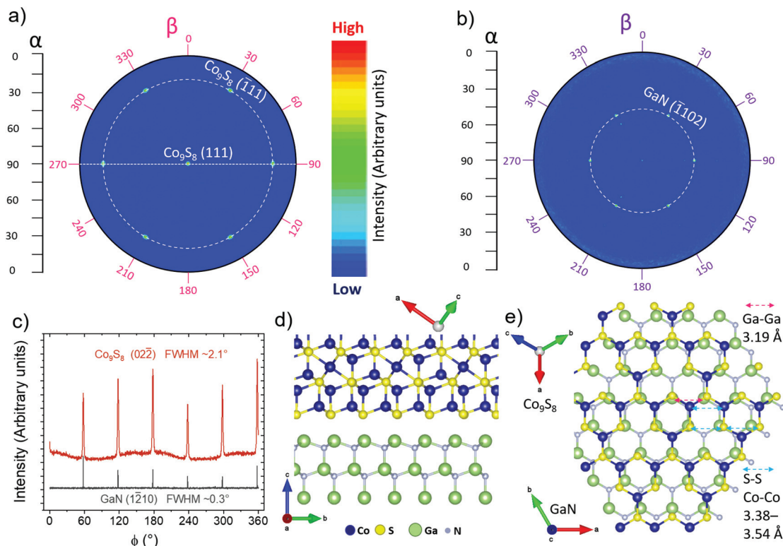
Fig. 5 In-plane pole figures at (a) 15.5^\circ 2\theta showing the out-of-plane (111) \text{Co}_9\text{S}_8 reflection in the middle ( 90^\circ\alpha ) and ( \bar{1}\bar{1}\bar{1} ) reflections tilted by 70.5^\circ ( 19.5^\circ\alpha ) and (b) 48.27^\circ 2\theta showing the ( \bar{1}\bar{1}02 ) \text{GaN} reflections at 47^\circ\alpha . Both pole figures were measured with the sample in the same orientation. (c) In-plane \phi scans of (022) \text{Co}_9\text{S}_8 ( 25.35^\circ 2\theta ) and ( \bar{1}210 ) \text{GaN} ( 57.95^\circ 2\theta ) reflections. The data has been vertically offset for clarity. Schematic of a possible epitaxial arrangement (111)[011] \text{Co}_9\text{S}_8 ||[(0001)[2 \bar{1}\bar{1} 0] \text{GaN} : (d) cross-sectional and (e) top view. In top view, only one puckered Co–S “layer” is shown for clarity. Selected atomic distances are indicated.
