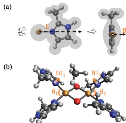
Fig. 2 (a) An illustration of Sterimol parameters for imidazole N-donor substituted with \text{CH}_3 , where L is length of the group along a user-defined axis ( \text{Cu-N} ) and B1 is the minimum width when looking down from the axis. The third Sterimol parameter, which is the corresponding maximum width, B5 , is not shown here. (b) Representation of strain descriptors \theta and B1 in IS . All strain descriptors are calculated using optimized IS geometries. (Cu: ochre, O: red, N: blue, C: grey).
