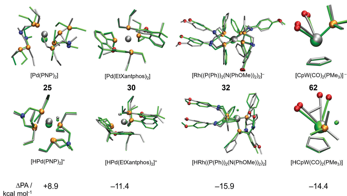
Fig. 5 Structure overlay plots of acid and base forms of some selected TM complexes optimized using GFN2- \chi TB (silver) and DFT (green). The top row shows conjugate base forms, while the bottom row shows the acid forms of complexes 25, 30, 32 and 62.
