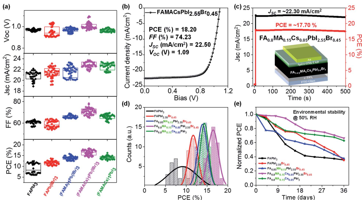
Fig. 4 Solar cell architecture and characterization. (a) Statistics of 30–40 devices for each FA 1-x-y MA x Cs 0.05 PbI 3-z Br z perovskite solar cell. (b) J - V curve for a peak efficiency of 18.20% obtained in the FA 0.8 MA 0.15 CS 0.05 PbI 2.55 Br 0.45 perovskite solar cell under AM 1.5G illumination. (c) The stabilized power output of J_{\text{SC}} and PCE is monitored over time at the maximum power point with the solar cell architecture. (d) Comparison of photovoltaic PCE distribution employing blade coated perovskite solar cells prepared at 150^\circ \text{C} (approximately 30–40 devices for each composition were measured). (e) Recorded long-term environmental stability of the corresponding FAPbI 3 , FAPbI 2.55 Br 0.45 , FA 0.85 MA 0.15 PbI 2.55 Br 0.45 , FA 0.8 MA 0.15 CS 0.05 PbI 2.55 Br 0.45 , and FA 0.8 MA 0.15 CS 0.05 PbI 3 perovskite solar cells exposed to an ambient environment with 50% relative humidity without encapsulation.
