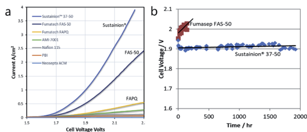
Fig. 9 (a) Comparison of current–voltage response of AEM electrolysis with various membranes in ref. 119. (b) Steady state voltage response at 1 \text{ A cm}^{-2} with Sustainion 37–50 membrane and FAS-50 membrane ( 60^\circ\text{C} , 1 \text{ M KOH} , \text{NiFe}_2\text{O}_4 anode and \text{NiFeCo} cathode). Reprinted from ref. 125 with permission from Elsevier. 125
