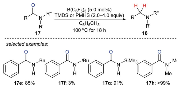
Scheme 16 Deoxygenation of amides catalysed by \text{B}(\text{C}_6\text{F}_5)_3 with TMDS or PMHS as reductants.
