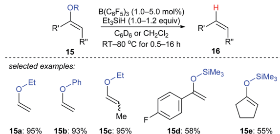
Scheme 14 Selective deoxygenation of enol ethers catalysed by \text{B}(\text{C}_6\text{F}_5)_3 with \text{Et}_3\text{SiH} as the reductant.
