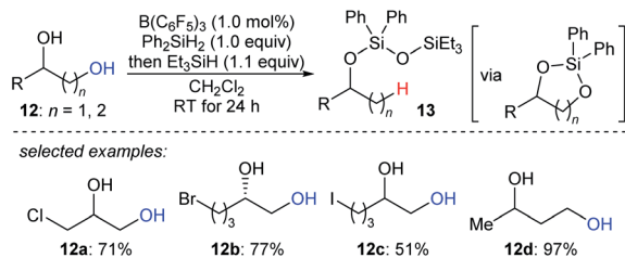
Scheme 12 Selective deoxygenation of terminal 1,2- and 1,3-diols catalysed by \text{B}(\text{C}_6\text{F}_5)_3 with \text{Et}_3\text{SiH} as the reductant.
