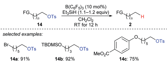
Scheme 13 Selective deoxygenation of primary alkyl tosylates catalysed by \text{B}(\text{C}_6\text{F}_5)_3 with \text{Et}_3\text{SiH} as the reductant.
