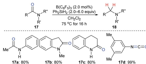
Scheme 15 Deoxygenation of amides and isocyanate catalysed by \text{B}(\text{C}_6\text{F}_5)_3 with \text{Ph}_2\text{SiH}_2 as the reductant.
