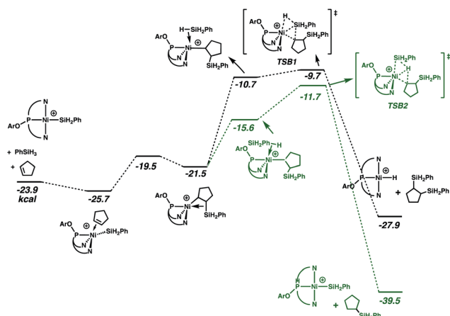
Fig. 3 Gibbs energy profile (kcal mol ^{-1} ) for cycle B of the hydrosilylation catalyzed by [(NPN)NiSiH_2Ph]^+ .
