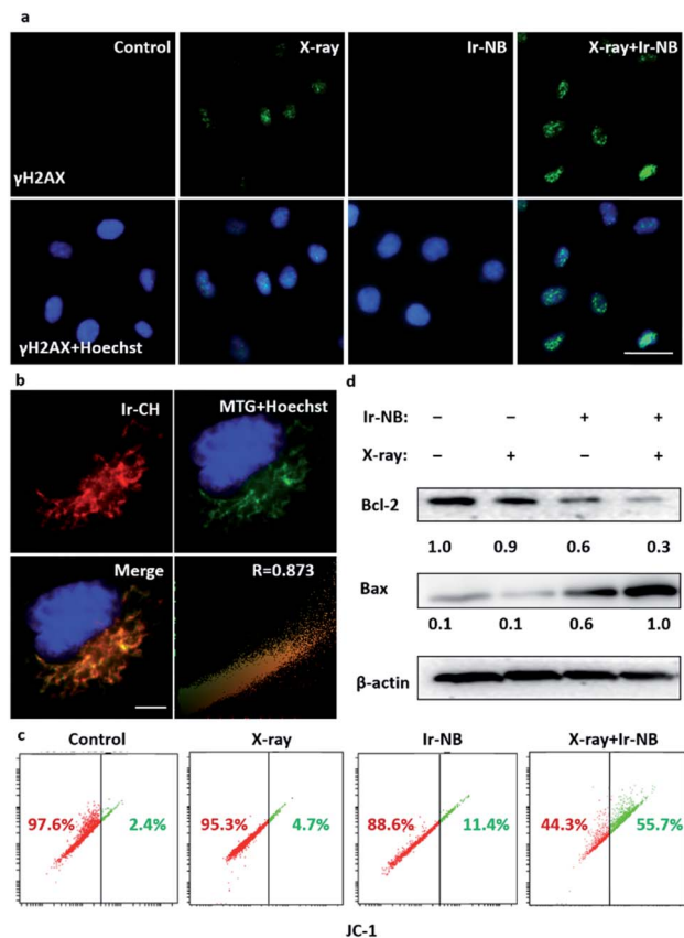
Fig. 4 Mitochondria-targeting iridium RS triggered loss of mitochondrial membrane potentials (MMP) inducing a synergetic effect on anticancer activity. (a) The expression of \gamma H2AX in A549 cells after treatment with Ir-NB and X-rays (4 Gy) was visualized using an immunofluorescence stain. Scale bar = 50 \mu m. (b) Fluorescent image of A549 cells labeled with Ir-CH ( \lambda_{ex} = 530, \lambda_{em} = 650–680 nm), Mito-Tracker green ( \lambda_{ex} = 490, \lambda_{em} = 510–530 nm) and Hoechst 33324. Scale bar = 10 \mu m. (c) The loss of mitochondrial membrane potential caused by the X-rays and Ir complex was measured by JC-1 flow cytometric analysis. (d) Expressed levels of Bcl-2 and Bax protein in A549 cancer cells after various treatments, and equal loading was verified by analysis of \beta -actin in the protein extracts.
