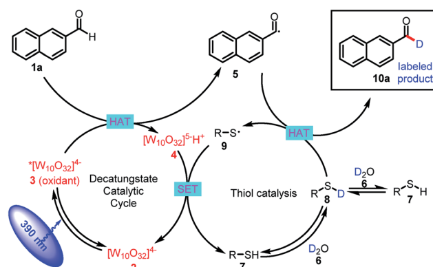
Scheme 2 Proposed mechanism.
