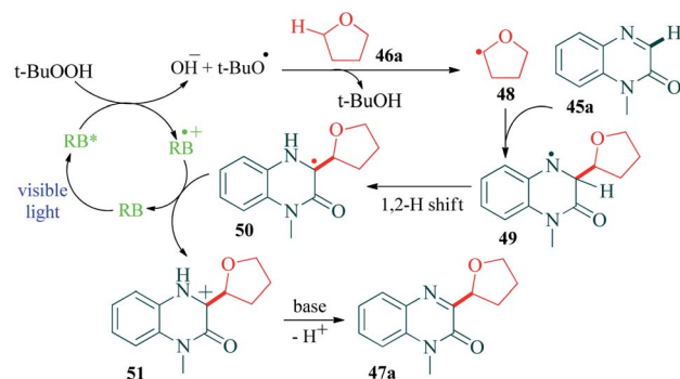
Scheme 14 Rose Bengal catalysed C–H/C–C cross-dehydrogenative-coupling.
