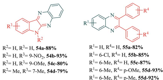
Scheme 15 Rose Bengal catalyzed synthesis of quinoxalines.
