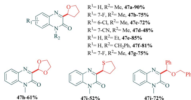
Scheme 13 Visible light promoted 3-oxyalkylation of quinoxalin-2(1 H )-ones.
