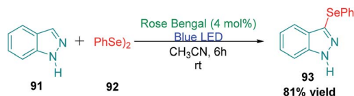
Scheme 27 Rose Bengal catalyzed selenylation of indazoles.
