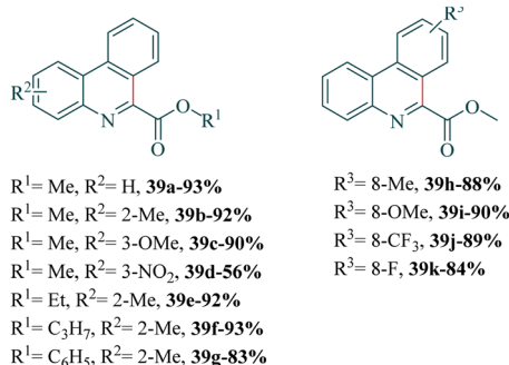
Scheme 11 Oxidative radical cyclization of N -biaryl glycine esters to phenanthridines.
