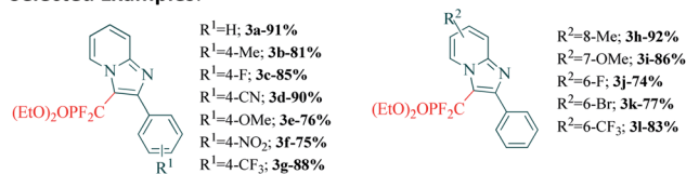
Scheme 1 Visible light promoted difluoromethylene-phosphonation of imidazoheterocycles.
