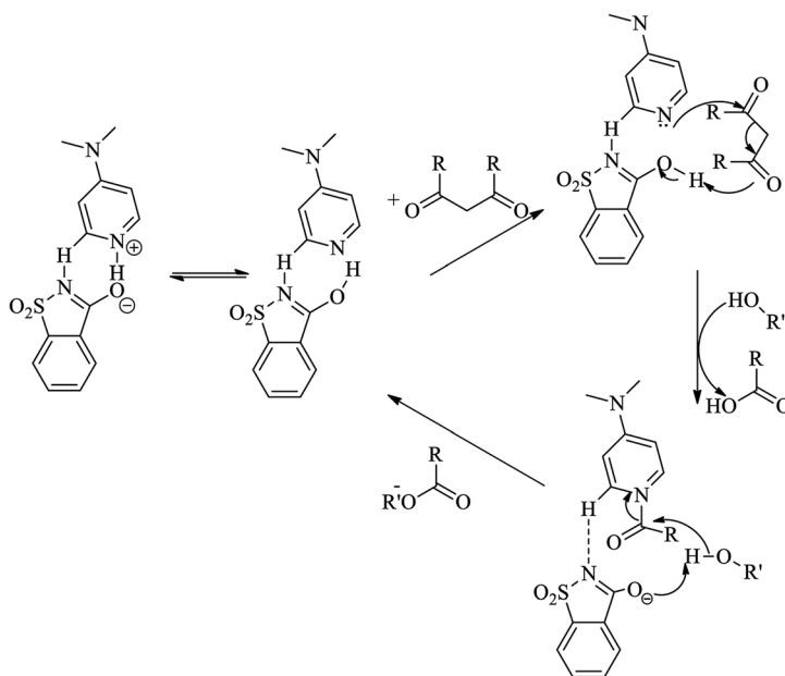
Scheme 99 Mechanism of DMAP catalyzed acylation reaction based on synthon connectivity as the resting state with O(\text{sac}) \cdots \text{HeN}(\text{py}) / O(\text{sac}) - \text{H} \cdot \text{N}(\text{py}) for propagation.
