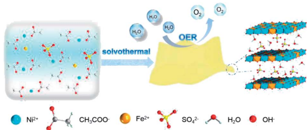
Scheme 1 Synthetic procedure for U-LDH( \text{SO}_4^{2-} ) nanosheets and its application in oxygen evolution reaction (OER).
