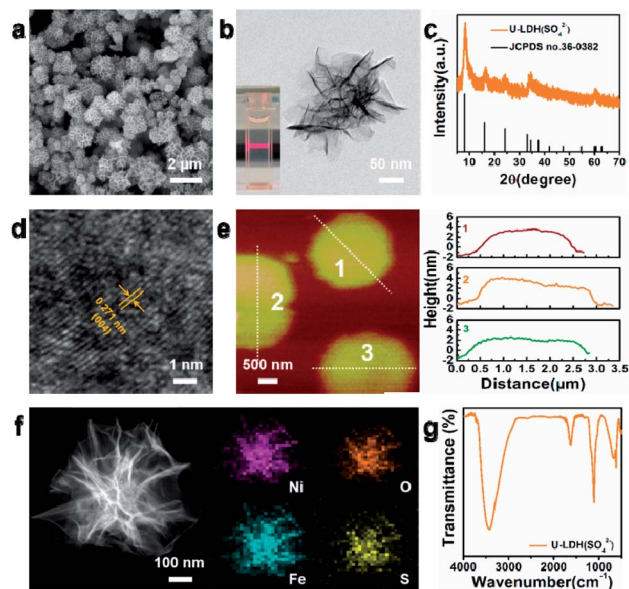
Fig. 1 (a) SEM image, (b) TEM image, (c) PXRD patterns, (d) HRTEM image, (e) AFM image and height profiles, (f) HAADF-STEM image and EDX elemental mappings, (g) FT-IR spectrum of the U-LDH( \text{SO}_4^{2-} ). The inset in (b) shows the Tyndall light scattering of the U-LDH( \text{SO}_4^{2-} ) in aqueous solution.
