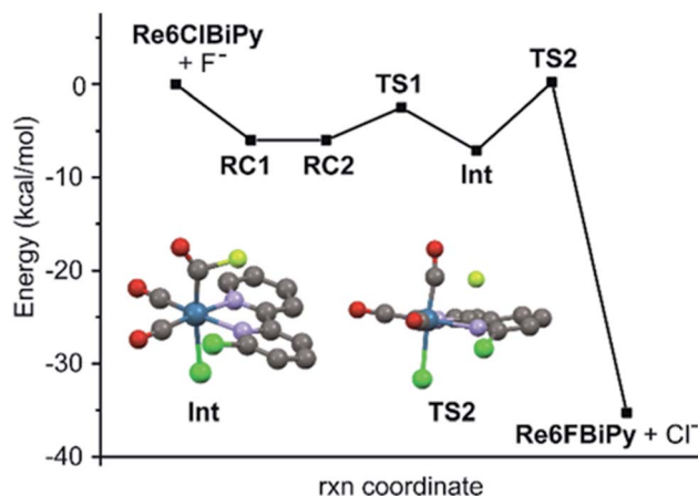
Fig. 7 DFT modelling of the reaction mechanism forming [\text{Re}(\text{CO})_3(-\text{L1h})\text{Cl}] ( \text{Re}_6\text{FBiPy} ) from [\text{Re}(\text{CO})_3(\text{L1b})\text{Cl}] ( \text{Re}_6\text{ClBiPy} ). The energies for the optimized geometries of the acyl fluoride intermediate species (Int) and the rate-determining transition states (TS) are plotted along the reaction coordinate.
